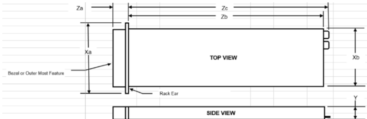
Figure 32. Chassis dimensions
